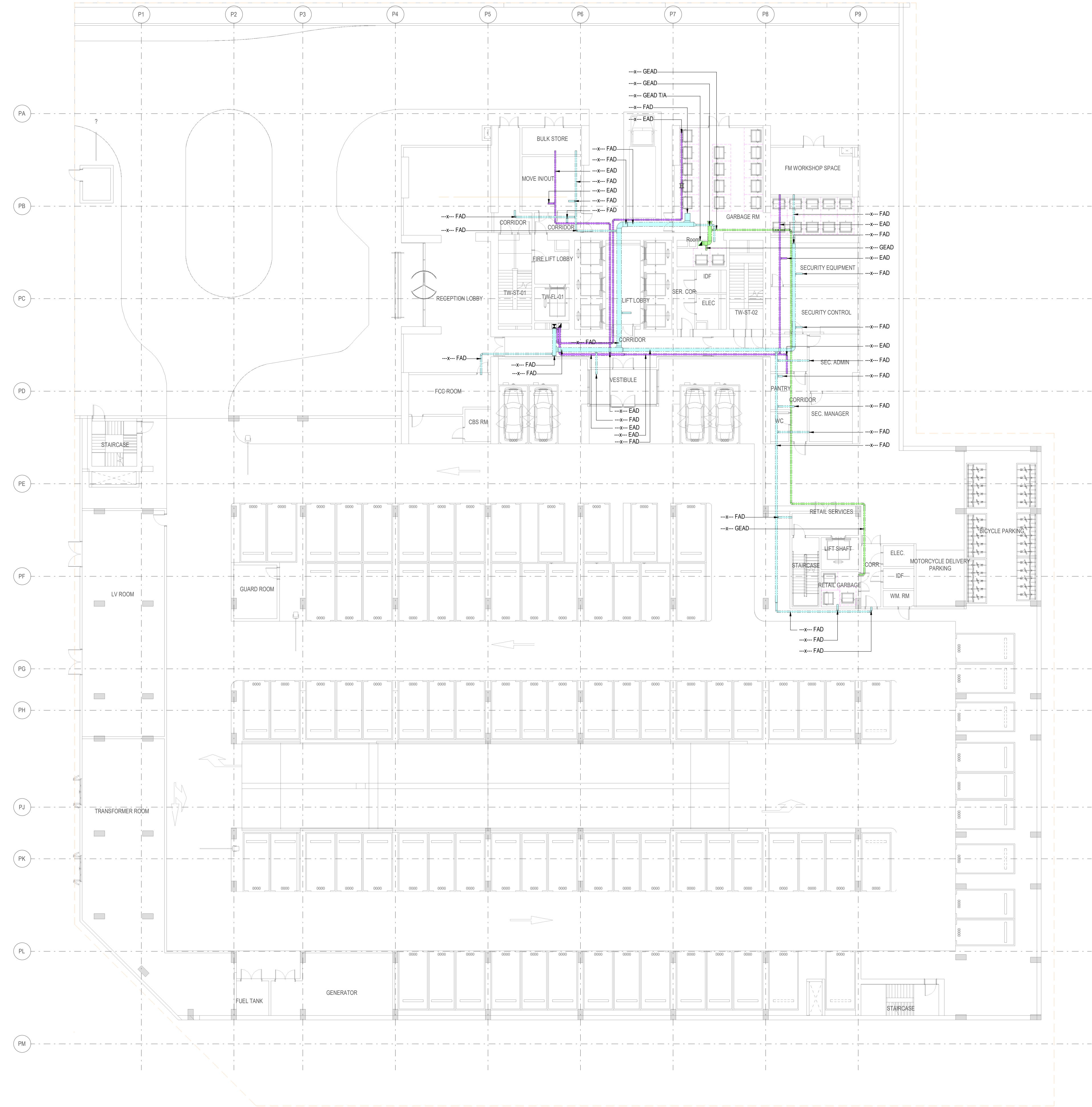
1 GROUND FLOOR VENTILATION SYSTEM SERVICES SPACE PLANNING & LAYOUT 2003 1 : 200
